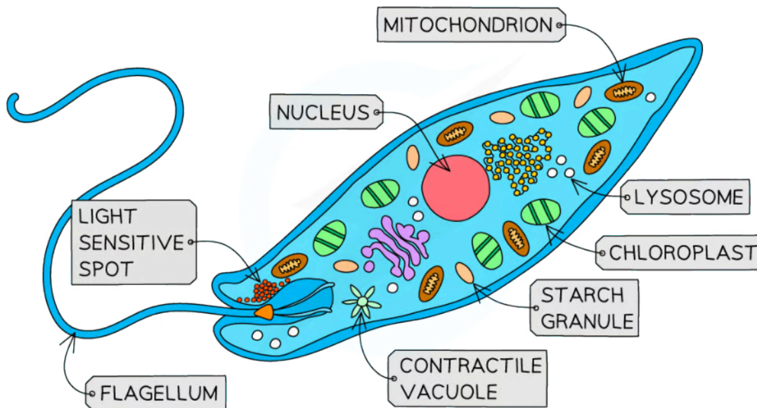
Euglena diagram
